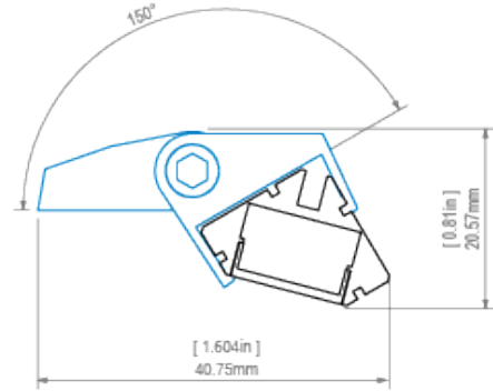
45-16 profile and REG-PD-UV mounting bracket profil 45-16 z mocownikiem REG-PD-UV
